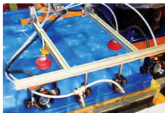
Model 8192 Gen4 Ion Air Cannons provide static elimination in between solar panel lenses to assist separation of the lenses during production.
